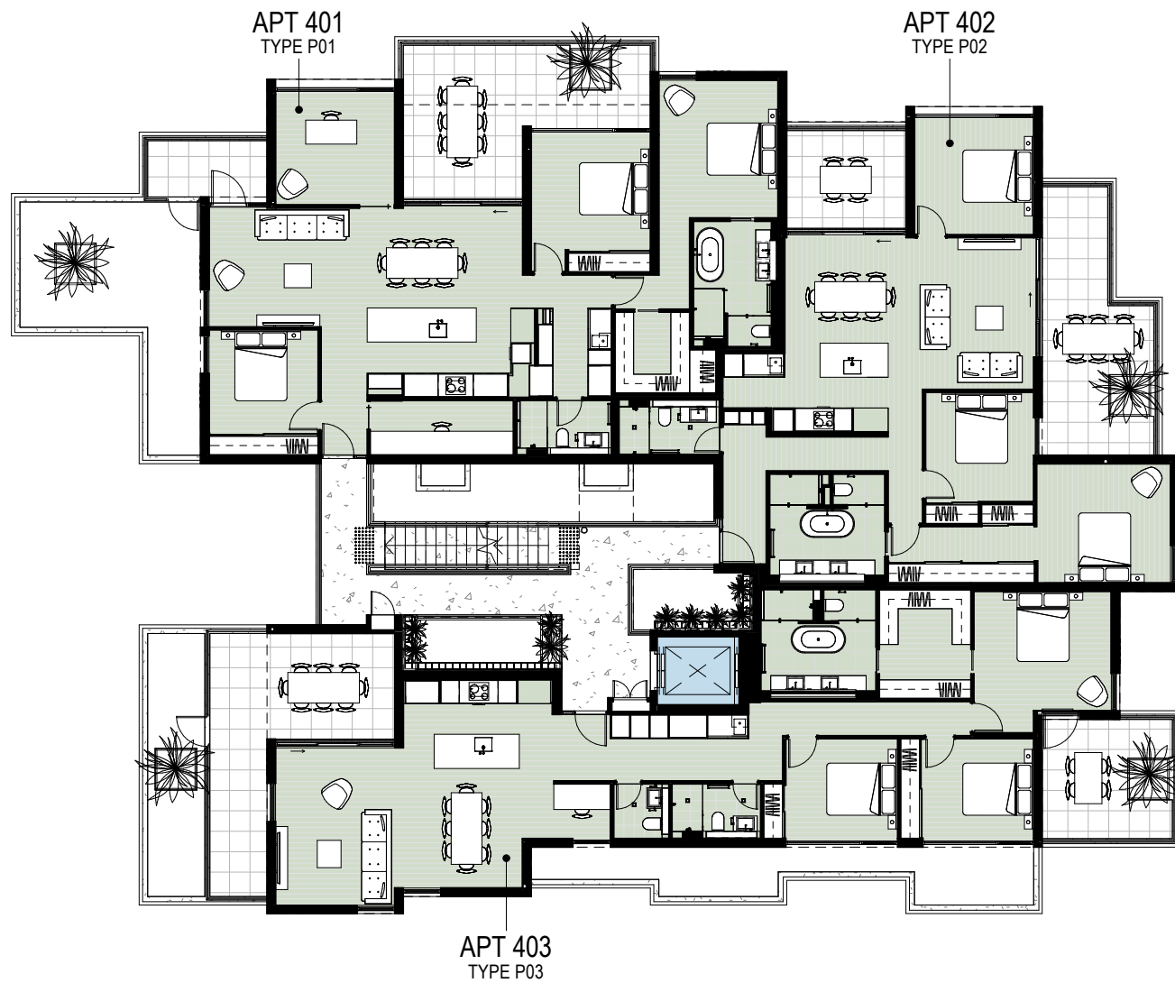
LEVEL 4 FLOOR PLAN
